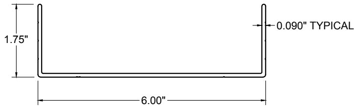
CHANNEL CROSS-SECTION
