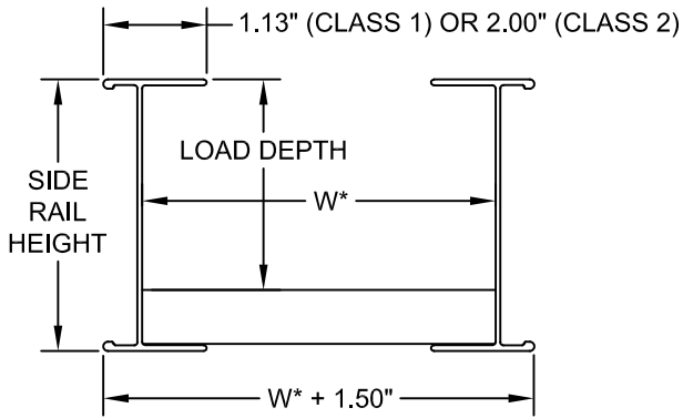
TRAY CROSS-SECTION
